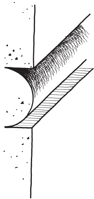
Bocel Corrido Flush Bed
